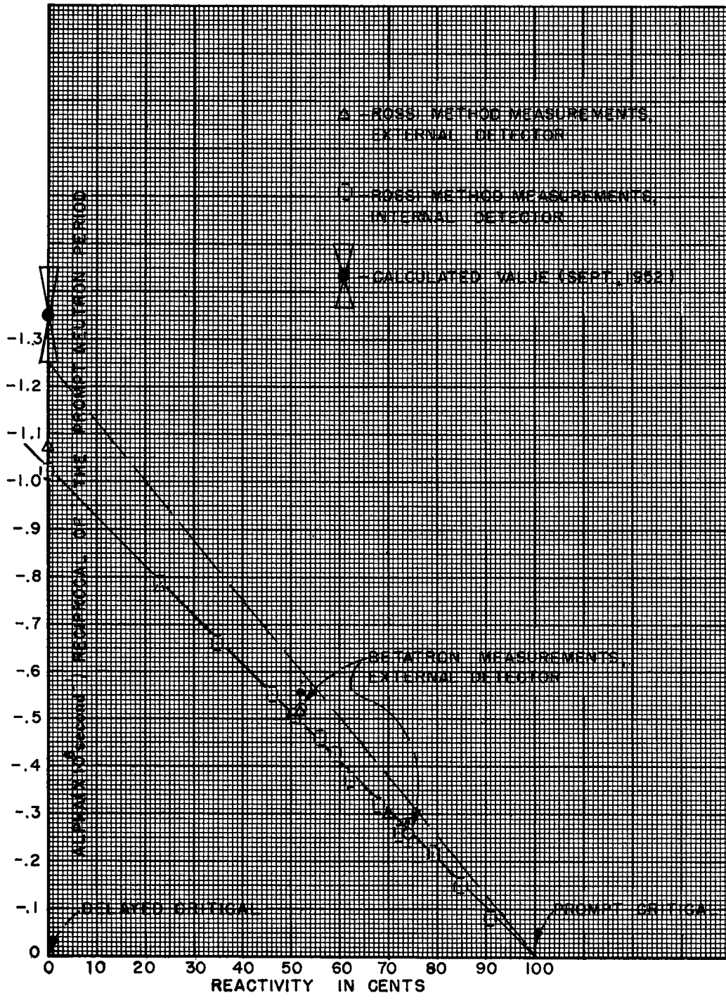
Fig. 7. Measurements of alpha on the Godiva critical assembly.
