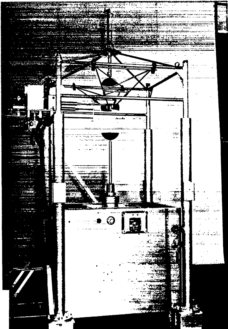
Fig. 1. The Godiva critical assembly, disassembled. The mechanism at the left operates control rods and source holder.
