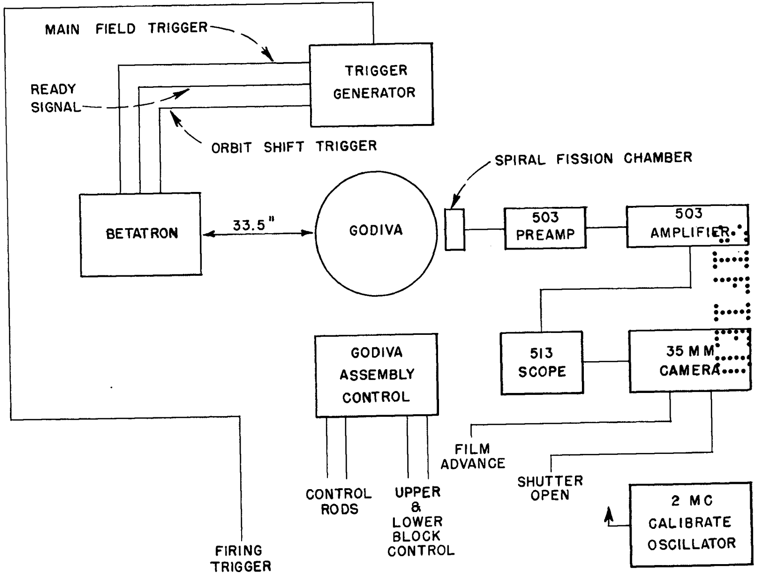
Fig. 2. Block diagram of the experimental arrangement used for making alpha measurements with a betatron.
