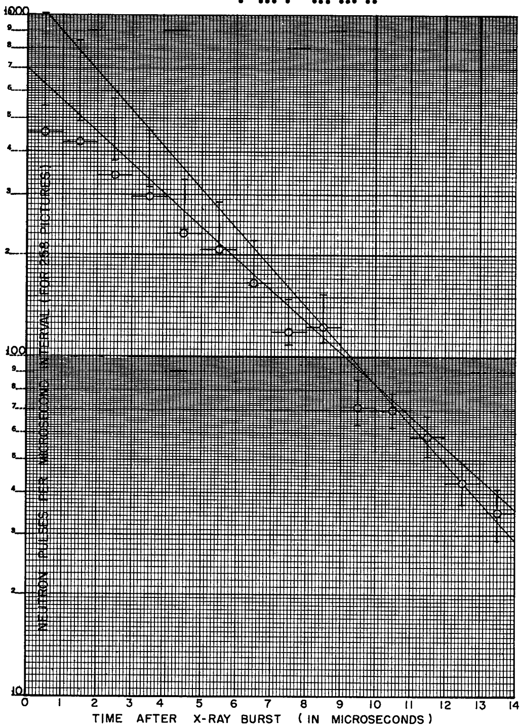
Fig. 6. Histogram of the number of pulses counted per microsecond with the critical assembly at 73.9 cents reactivity.
